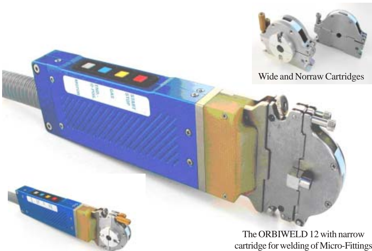
The ORBIWELD 12 with wide cartridge for normal applications
